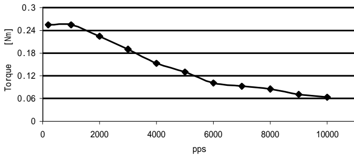
BL42STH47-1206MA VM: 24VDC; 1.2A /相 驱动器: HA335, 整步
