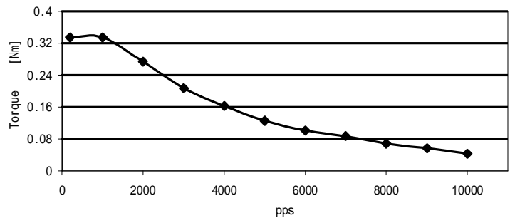
BL42STH47-1684MA VM: 30VDC; 1.77A /相 驱动器: HA335, 整步
